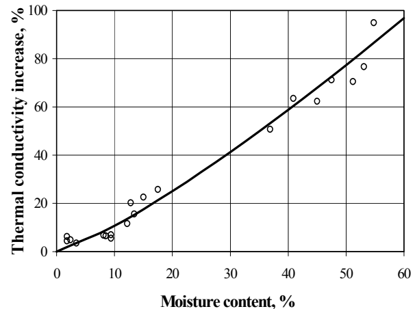
Fig. 1. The dependence of thermal conductivity increase on moisture content of cellulose insulation
