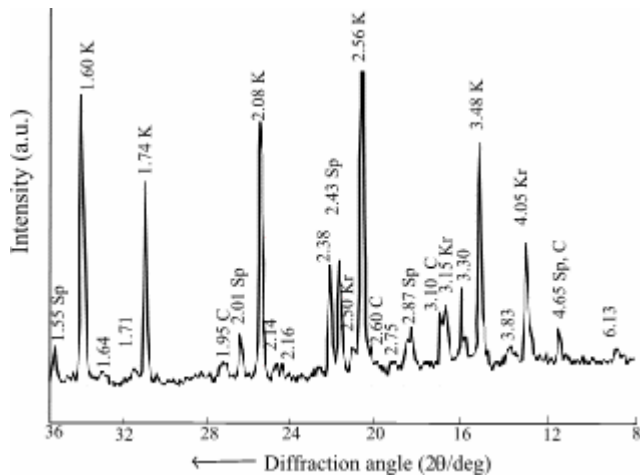
Fig. 3. X-ray diffraction pattern of the waste catalyst at burning temperature 1100 °C (notation index is presented in the text)
