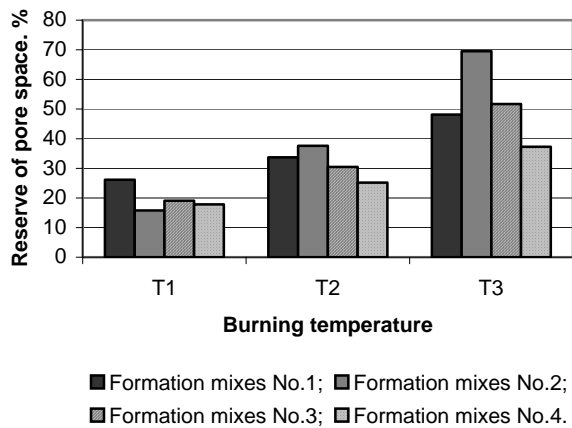
Fig. 7. Dependence of reserve of pore space the burning temperature
