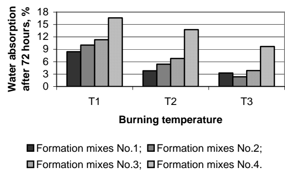
Fig. 6. Dependence of water absorption after 72 hours on the burning temperature
