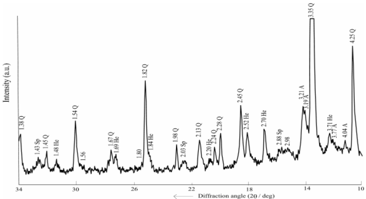
Fig. 9. X-ray diffraction pattern of samples of the ceramics body without of catalyst additives at burning temperature 1100 °C (notation index is presented in the text)
