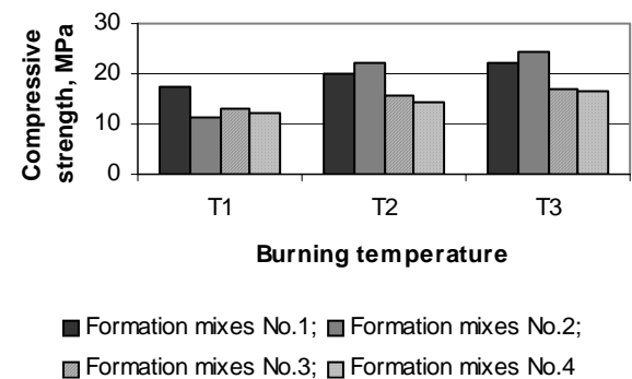
Fig. 5. Dependence of compressive strength on the burning temperature
