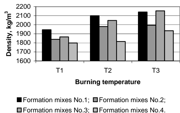
Fig. 4. Dependence of density on the burning temperature
