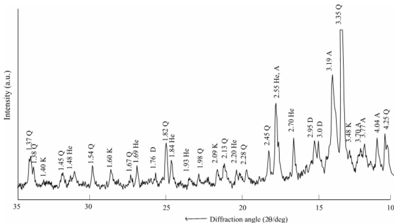
Fig. 10. X-ray diffraction pattern of examples of the ceramics body with 5 % of catalyst additives at burning temperature 1100 °C (notation index is presented in the text)
