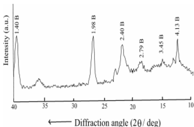
Fig. 2. X-ray diffraction pattern of the waste catalyst at burning temperature 1000 °C (notation index is presented in the text)
