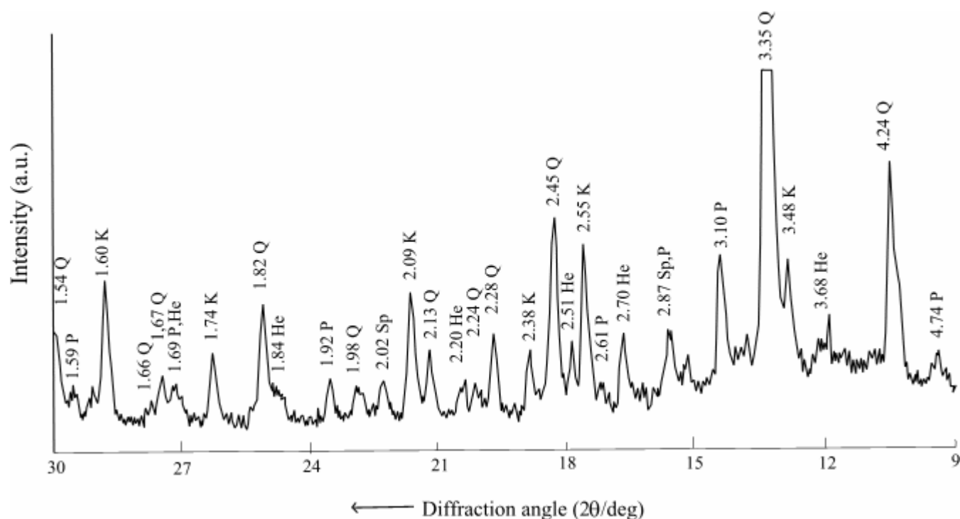
Fig. 11. X-ray diffraction pattern of examples of the ceramics body with 20 % of catalyst additives at burning temperature 1100 °C (notation index is presented in the text)
