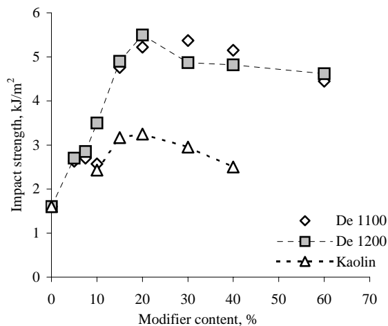
Fig. 1. Effect of modifier content on the impact strength
