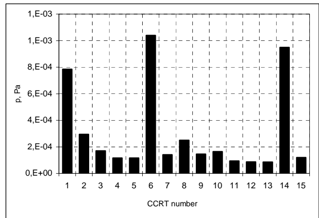
Fig. 6. The distribution of total pressures within A33EKC CCR tubes
