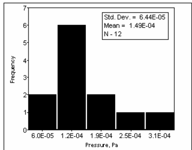
Fig. 7. Histogram of 12 A33EKC CCR tubes total pressures
