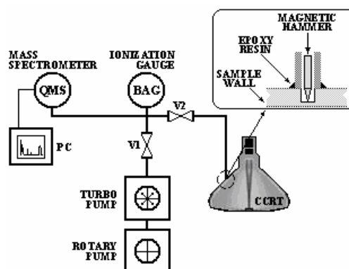
Fig. 1. Experimental set-up for RGA on CCRTs. PC – personal computer, V1 and V2 – valves, QMS – quadrupole mass spectrometer, BAG – Bayard-Alpert ionization gauge
