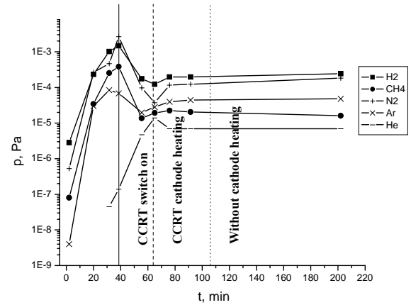
Fig. 4. Residual gases (H 2 , CH 4 , N 2 , Ar, He) partial pressures dependence on time
