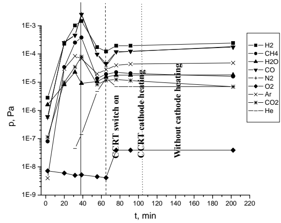
Fig. 3. Typical residual gas partial pressure dependence on time
