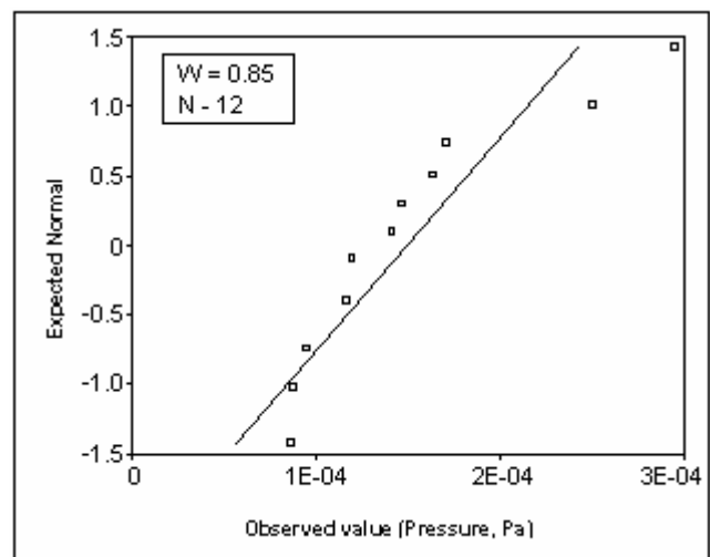
Fig. 8. Normal plot of 12 A33EKC CCR tubes total pressures
