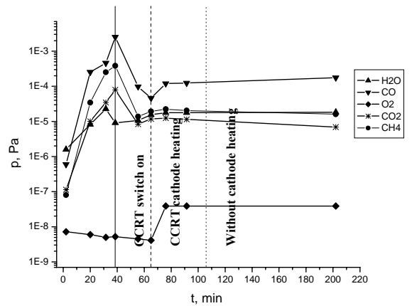
Fig. 5. Residual gases (H 2 O, CO, CO 2 , CH 4 ) partial pressures dependence on time
