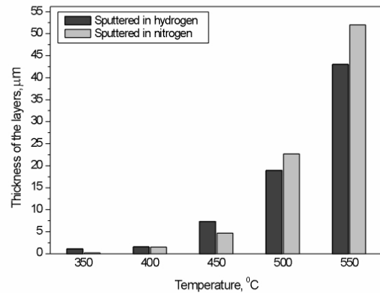
Fig. 6. Thickness of the layers depending on the sputtering and gas nitriding parameters.
