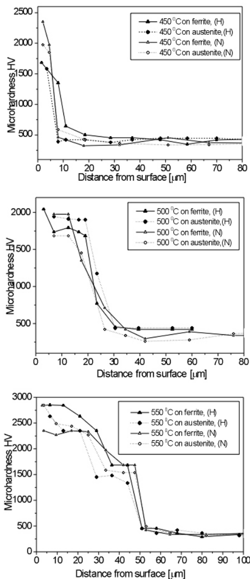
Fig. 8. Microhardness profiles of the samples nitrided in various treatment conditions
