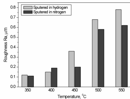
Fig. 7. Roughness of the samples after gas nitriding
