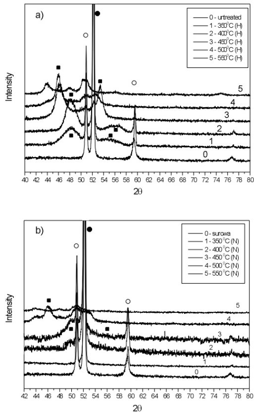
Fig. 2. Diffraction patterns for all the samples depending on the nitriding temperature and sputtering gas: a – sputtered in hydrogen (H); b – sputtered in nitrogen (N)
