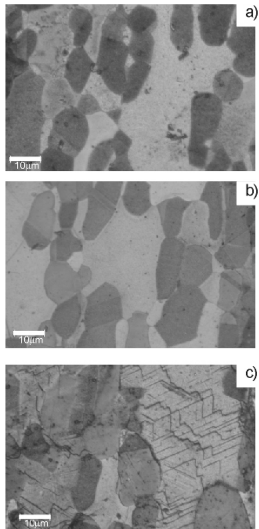
Fig. 3. Surface of the samples sputtered in nitrogen after nitriding at: a – 350 °C , b – 400 °C , c – 450 °C
