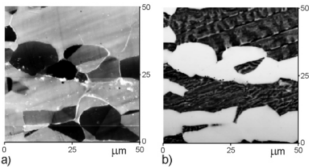
Fig. 1. AFM (a) and MFM (b) image of the surface of duplex steel. The darker regions in the right picture correspond to ferritic (magnetic) grains
