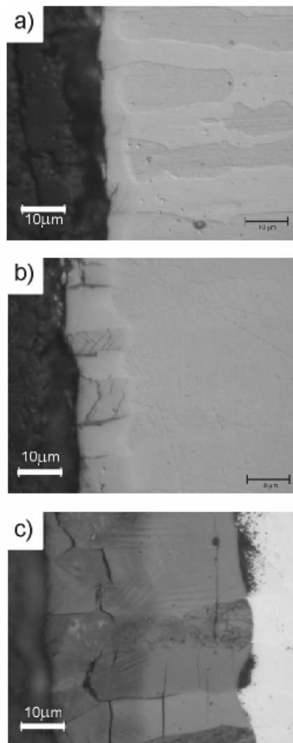
Fig. 9. Pictures of the cross-section of the layers obtained after nitriding at: a – 450 °C, b – 500 °C, c – 550 °C. Samples sputtered in hydrogen; LMA
