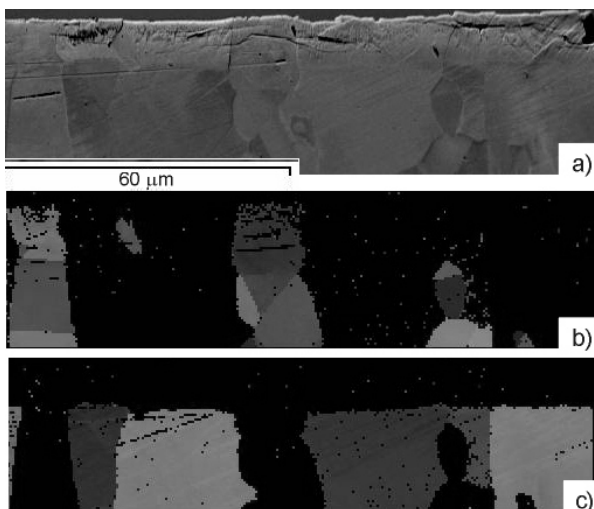
Fig. 5. EBSD picture of the layer produced during nitriding at 450 °C: a – SEM picture of the layer; b – austenite; c – ferrite identification
