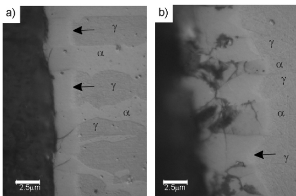
Fig. 4. Cross sections of the layers on duplex steel after nitriding at: a – 400 °C; b – 450 °C. The arrows shows the curvature of the layer on austenitic grains
