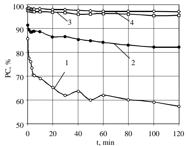
Fig. 7. Dependence of print contrast level on the wearing duration in the case of digital prints: 1 – Ensobulky paper, 2 – Offset paper, 3 – Gloss paper, 4 – Silk paper
