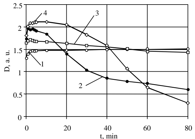
Fig. 2. Dependence of optical density on the wearing duration after a cyclic temperature change: 1 – direct thermography: paper KLS-44, heating head temperature R25 , printing speed v_{sp} = 0.102 m/s; 2 – indirect thermography: paper PP White, ink transfer ribbon Wax, R30 , v_{sp} = 0.051 m/s; 3 – indirect thermography: paper COAT PC, ink transfer ribbon Wax, R30 , v_{sp} = 0.051 m/s; 4 – indirect thermography: paper COAT PC, ink transfer ribbon Wax, R30 , v_{sp} = 0.051 m/s; v_1 = 0.47 m/s, P = 441.45 \times 10^{-3} N/cm 2
