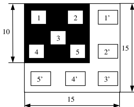
Fig. 1. Scheme of experimental areas for studying resistance of the prints and the base to mechanical wear: 1–5 are the points where the optical density of the print was measured, 1'–5' are the points where the optical density of the base was measured
