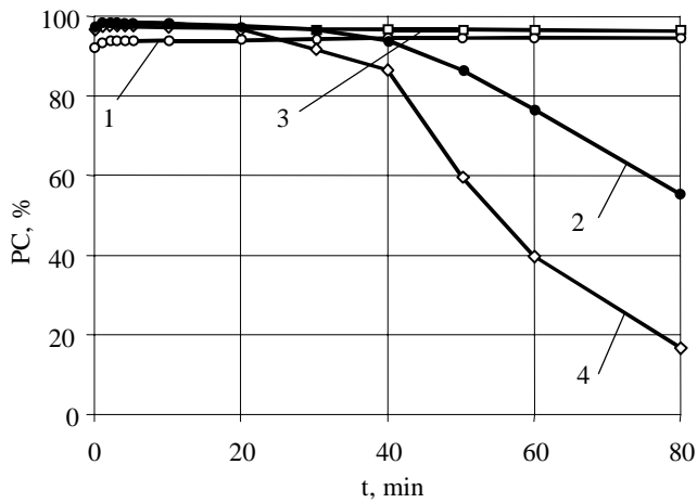
Fig. 3. Dependence of printing contrast level on the wearing duration: 1 – direct thermography: paper KLS-44, heating head temperature R_{25} , printing speed v_{sp} = 0.102 m/s; 2 – indirect thermography: paper PP White, ink transfer ribbon Wax, R_{30} , v_{sp} = 0.051 m/s; 3 – indirect thermography: paper PP White, ink transfer ribbon Resin, R_{30} , v_{sp} = 0.051 m/s; 4 – indirect thermography: paper COAT PC, ink transfer ribbon Wax, R_{30} , v_{sp} = 0.051 m/s; v_1 = 0.47 m/s, P = 441.45 \times 10^{-3} N/cm 2
