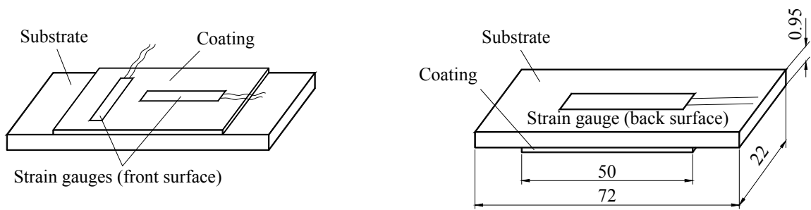
Fig. 4. Geometry of the specimen
