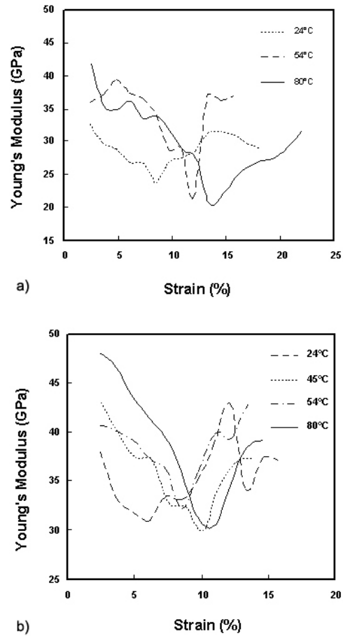
Fig. 4. Young's modulus vs. strain relationships of NiTi polycrystalline wires in heating (a) and cooling process (b)
