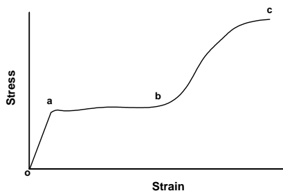
Fig. 1. Typical stress vs. strain relationship
