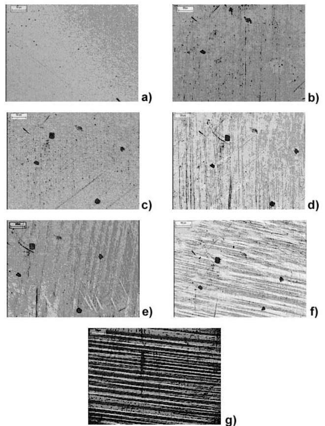
Fig. 7. Optical results: a – after polishing; b – 2 % strain; c – 4 % strain; d – 6 % strain; e – 8 % strain; f – 10 % strain; g – 11 % strain. Scale bar is 50\ \mu\text{m} . Refer to Fig. 6 for the location where the result was obtained
