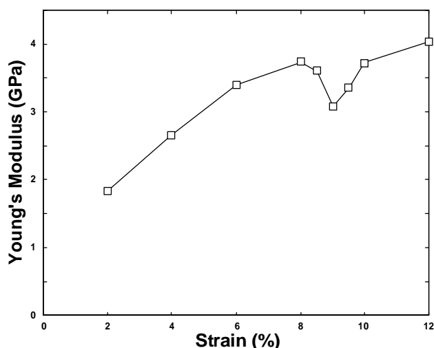
Fig. 8. Young's modulus vs. strain relationship of CuAlNi single crystal
