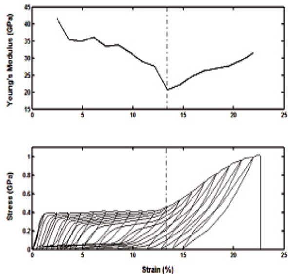
Fig. 5. Typical results of NiTi wires at 80 °C in heating process
