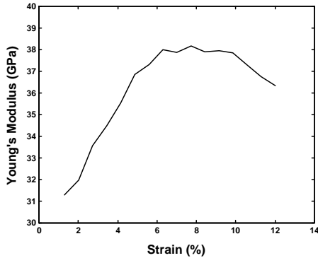
Fig. 3. Young's modulus vs. strain relationship of a NiTi polycrystalline wire (initially twinned martensite phase) [12]
