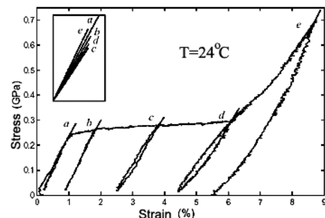
Fig. 2. Stress vs. strain relationship of a NiTi polycrystalline wire under cyclic tension (initially R-phase) and Young's modulus measured at a few points [6]
