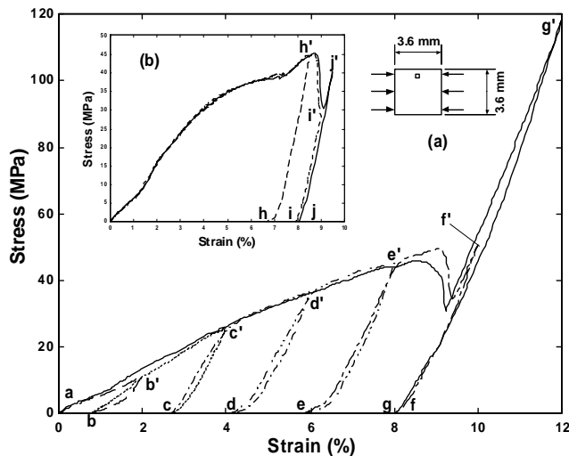
Fig. 6. Stress vs. strain relationship of CuAlNi single crystal [13]
