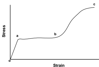
Fig. 1. Typical stress vs. strain relationship
