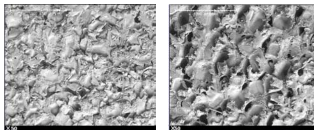
Fig. 8. SEM photos of 200 kg/m 3 density foam of undamaged (a) and damaged (b) specimens in indentation tests
