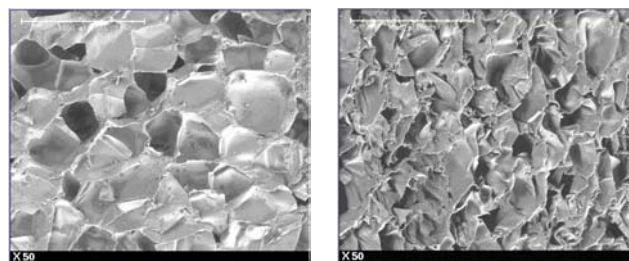
Fig. 7. SEM photos of 100 kg/m 3 density foam of undamaged (a) and damaged (b) specimens in indentation tests
