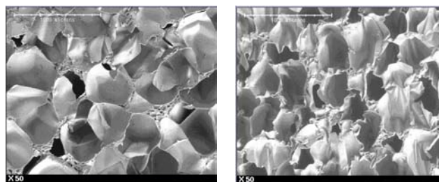
Fig. 6. SEM photos of 80 kg/m 3 density foam of undamaged (a) and damaged (b) specimens in indentation tests
