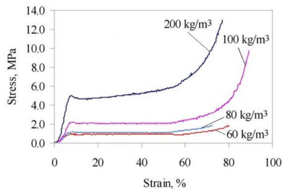
Fig. 1. Stress versus normalised displacement for four core densities in monotonic compression tests.
