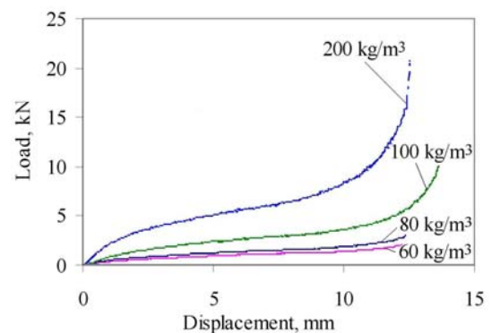
Fig. 2. Evolution of load versus displacement for foams of four densities in static indentation
