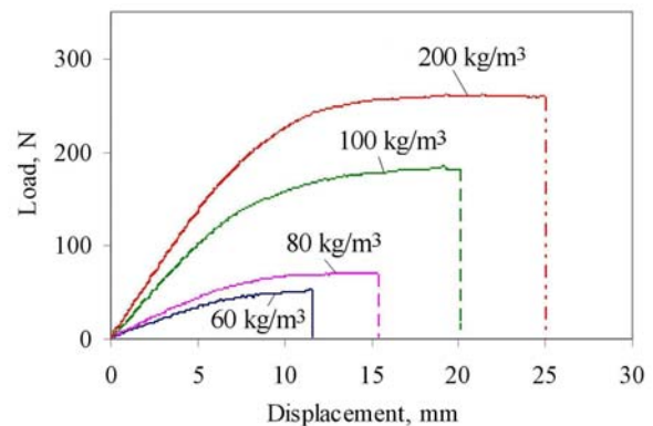
Fig. 4. Load displacement curves for cores of four densities in three point bending static tests
