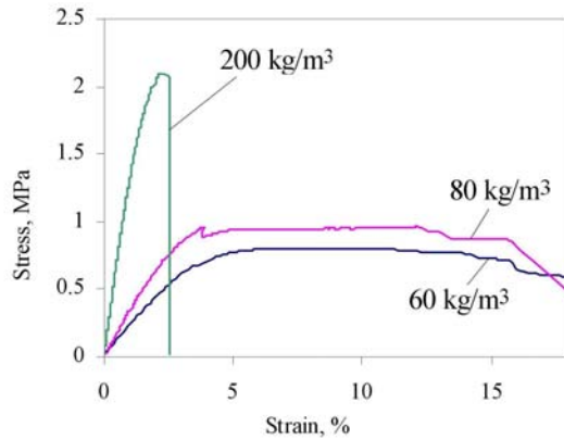
Fig. 3. Stress-strain curves of 60, 80 and 200 kg/m 3 densities foams in static shear tests
