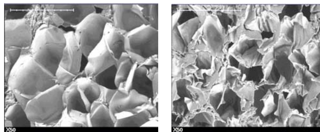
Fig. 5. SEM photos of 60 kg/m 3 density foam of undamaged (a) and damaged (b) specimens in indentation tests
