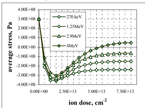
Fig. 1. Calculated dependence of the average stress in the \text{SiO}_2\text{-Si} system implanted with \text{Xe}^+ on the dose and energy of ions
