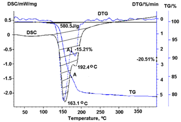
Fig. 1. TG-DTG-DSC curves of the Kovdor phosphogypsum. a – initial material, b – after 5 minutes of hydration, c – after 20 minutes of hydration, d – after 120 minutes of hydration
