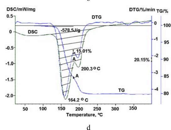
Fig. 2. TG-DTG-DSC curves of the Kirov phosphogypsum. a – initial material, b – after 3 days of hydration, c – after 14 days of hydration, d – after 105 days of hydration
