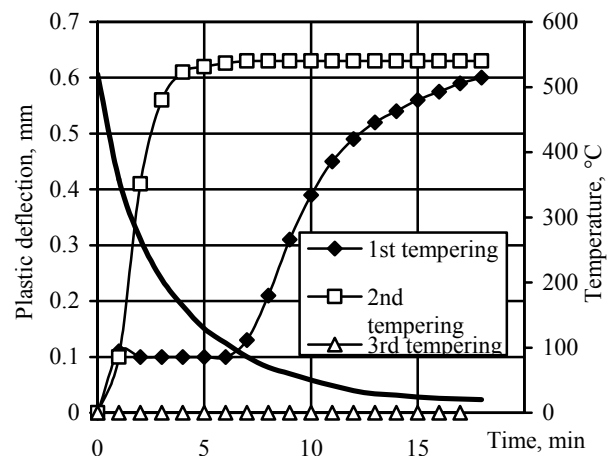
Fig. 2. Kinetics of the transformation plasticity change after repeated tempering and holding for 1 h at the temperature of 520 °C; \sigma_1 = 600 \text{ N/mm}^2 , steel Cr12V1
