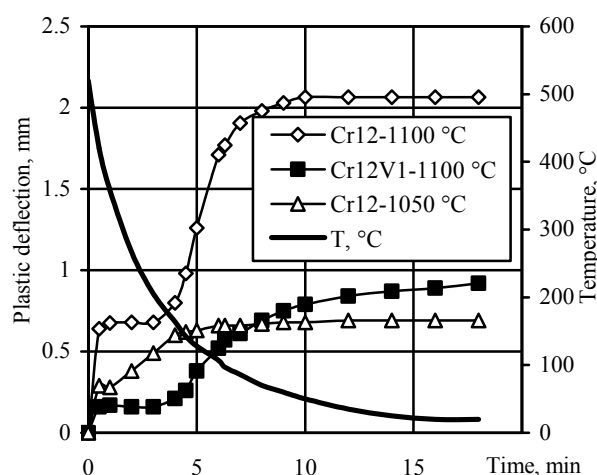
Fig. 1. Kinetics of the plastic deflection changes during cooling after the first tempering
