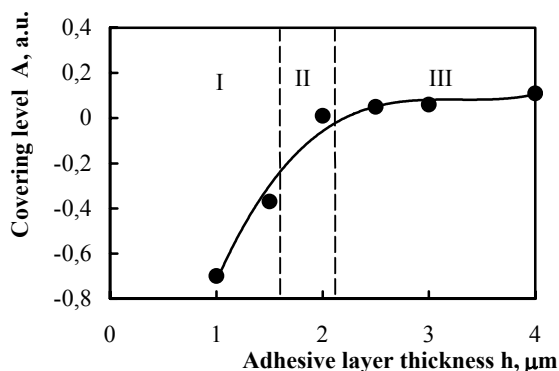
Fig. 2. The covering quality of hot stamped holographic foil vs adhesive layer thickness
