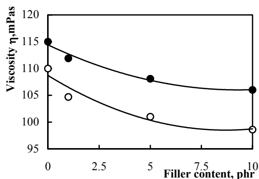
Fig. 1. The influence of filler content on viscosity \eta of VeoVa-10/MMA/2-EHA at different shear rate \dot{\gamma} , \text{s}^{-1} : \circ – 42, \bullet – 50
