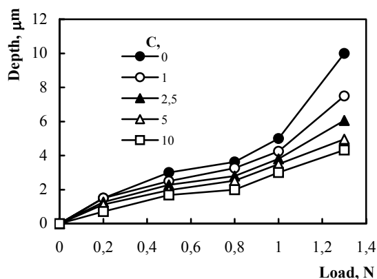
Fig. 5. The influence of scratch load on the groove depth for adhesive compositions modified with various amounts of \text{TiO}_2
