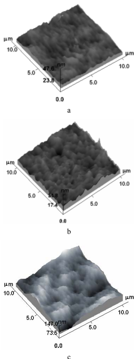
Fig. 4. AFM images of VeoVa-10/MMA/2-EHA adhesive surface topography filled with different content of \text{TiO}_2 : a – 0, b – 2.5 phr, c – 10 phr
