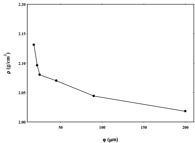
Fig. 1. Relationship between pycnometric density and average particle size of the ceramic sample I
