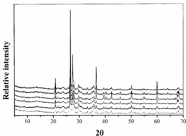
Fig. 3. X-ray diffraction patterns of the calcinated clay ceramic sample I from different granulometric fractions (from 18 \mu\text{m} to 200 \mu\text{m} )
