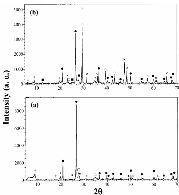
Fig. 4. X-ray diffraction patterns of the historical ancient pottery from: (a) Beniāičiai and (b) Turlojiškės .
