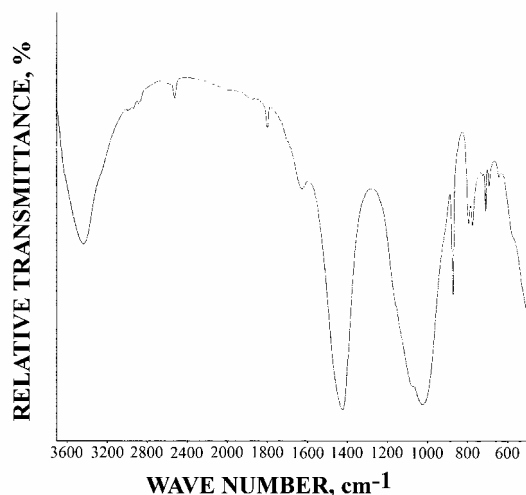
Fig. 6. IR spectrum of the historical ancient pottery from Turlojiškės
