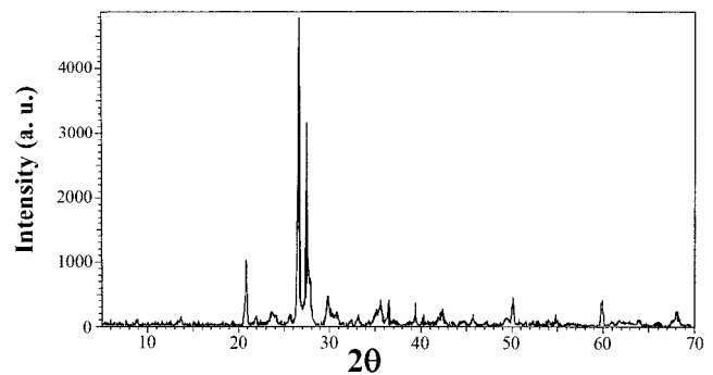
Fig. 2. X-ray diffraction pattern of the calcinated clay ceramic sample I from the granulometric fraction of 25 \mu\text{m}
