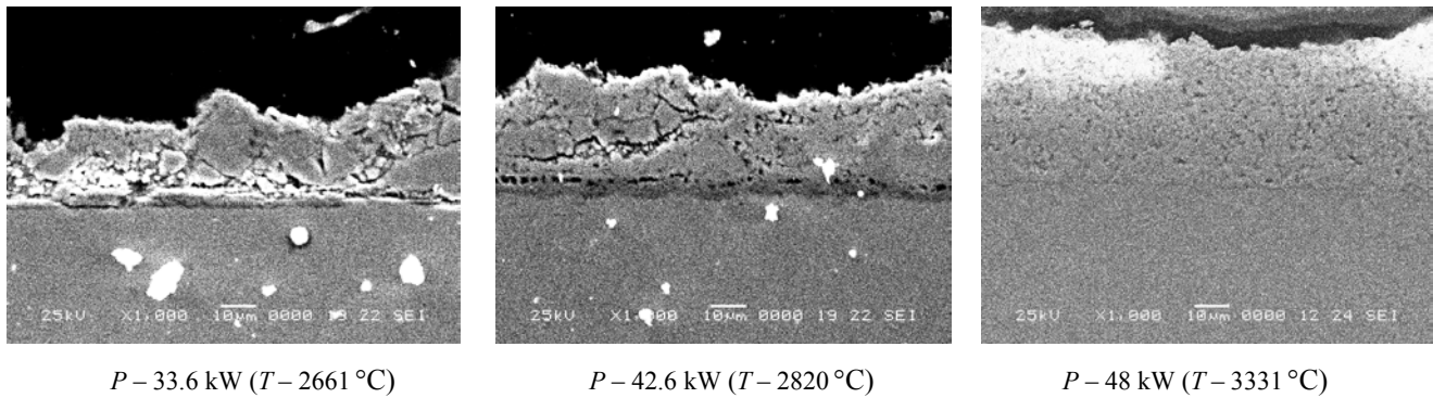
Fig. 8. Influence of P on plasma sprayed YSZ film properties. Regime C, x - 70 mm, started powder YSZ-2
