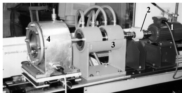
Fig. 2. Test rig for power consumption evaluation, 1 – electric motor, 2 – torquemeter, 3 – areostatic bearings 4 – test chamber
