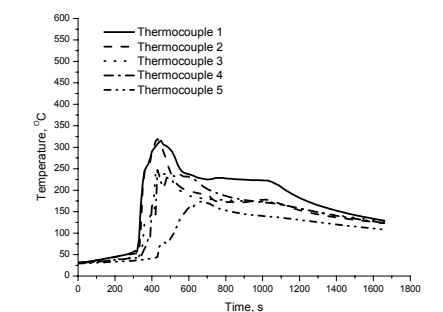
Fig. 10. Fragment 2.1 temperature changes
