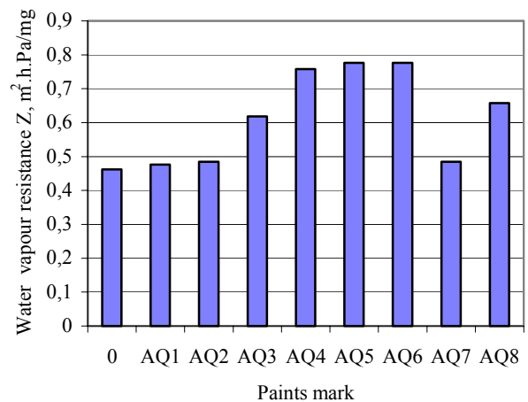
Fig. 1. Vapour resistances of surface layer of silicate brick coated with aqueous polymeric dispersion paints
