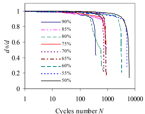
Fig. 3. Evolution of the stiffness of the KFRP laminates according to the number of cycles N for different applied load levels
