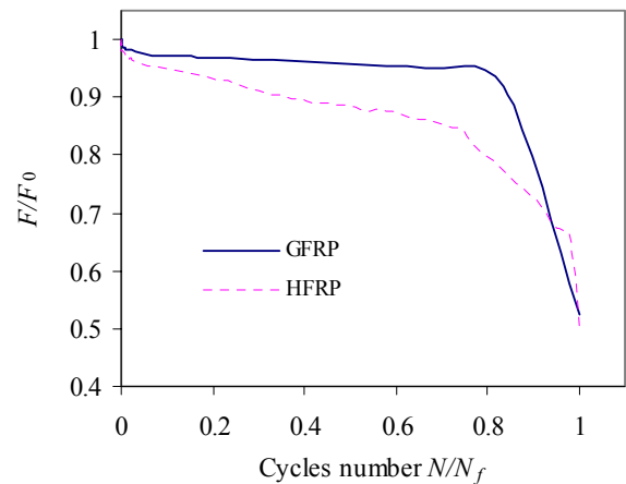
Fig. 5. Typical curves of the evolution of the load testing the glass (GFRP) and hybrid (HFRP) fibre laminates according to the number of cycles during fatigue test
