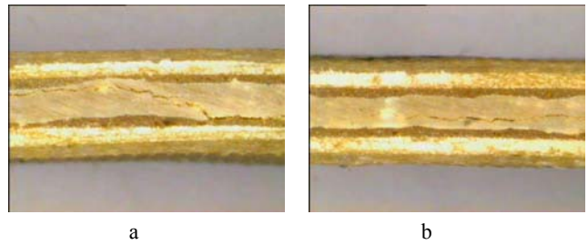
Fig. 11. Fractures on the frontal surfaces of the test-specimen in HFRP laminate after cyclic fatigue tests
