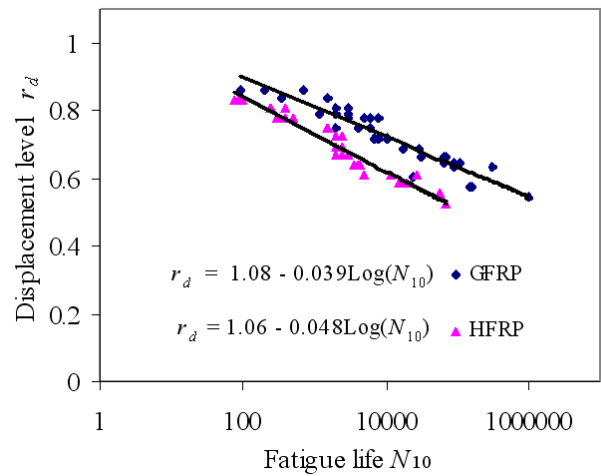
Fig. 13. Wöhler curves of the GFRP and HFRP laminates
