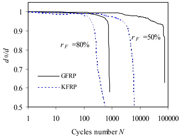
Fig. 4. Comparative study of GFRP and KFRP laminates for two applied load levels
