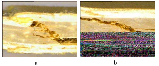
Fig. 10. Fractures on the frontal surfaces of the test-specimens in KFRP laminate after cyclic fatigue tests
