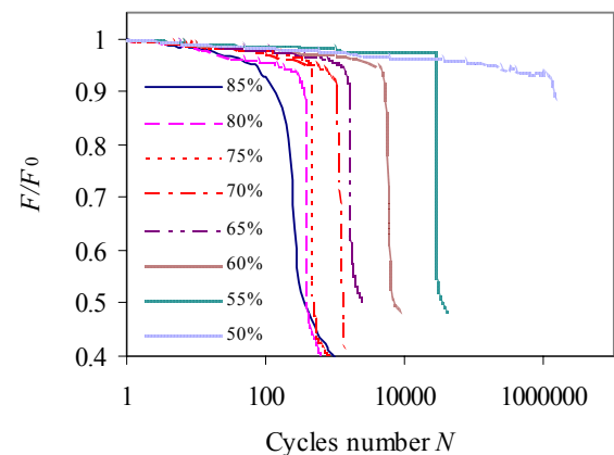
Fig. 6. Evolution of the load F/F_0 of glass fibres (GFRP) laminates according the number of N cycles
