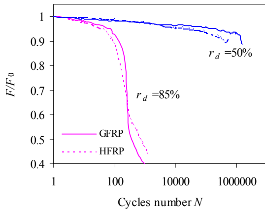
Fig. 8. Comparative study of GFRP and HFRP laminates for two applied displacement levels
