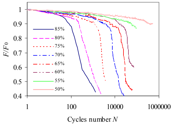
Fig. 7. Evolution of the load F/F_0 of hybrid HFRP laminates according the number of N cycles
