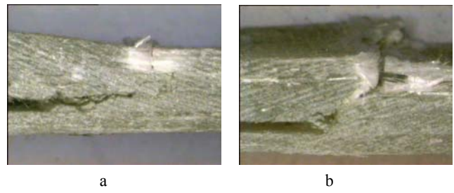
Fig. 9. Fractures on the frontal surfaces of the test-specimens in GFRP laminate after cyclic fatigue tests
