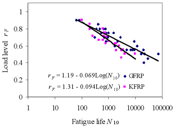
Fig. 12. Wöhler curves of the GFRP and KFRP laminates
