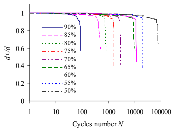
Fig. 2. Evolution of the stiffness of the GFRP laminates according to the number of cycles N for different applied load levels
