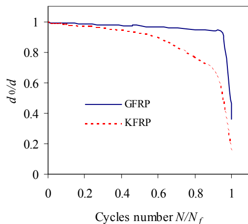
Fig. 1. Curve types of the evolution of stiffness according to the number of cycles
