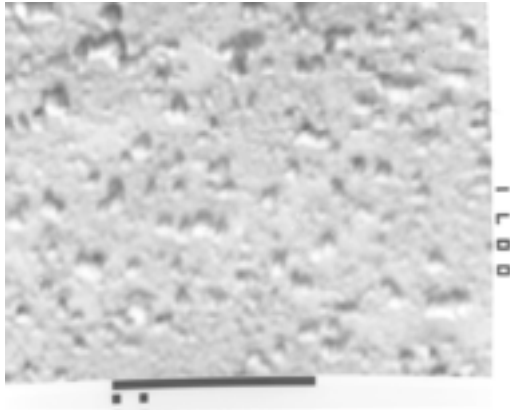
Fig. 7. SEM photograph of fine-dispersive fraction of the glacial lacustrine material in depth 40 – 50 cm (marker value 10 \mu\text{m} )
