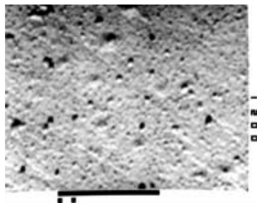
Fig. 1. SEM photograph of fine-dispersive fraction of the glacial lacustrine material in depth 0 – 10 cm (marker value 10 \mu\text{m} )
