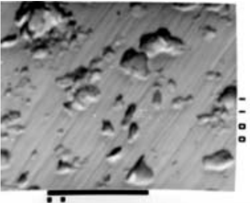
Fig. 3. SEM photograph of fine-dispersive fraction of the glacial lacustrine material in depth 10 – 20 cm (marker value 10 \mu\text{m} )
