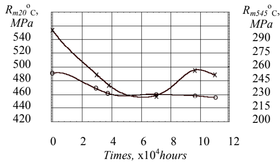
Fig. 5. Dependence of ultimate tensile strength on time of operation: o – the research was done at the 20 °C temperature, × – the researches was done at the 545 °C temperature
