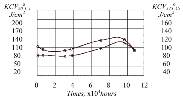
Fig. 9. Dependence of impact strength on time of operation: o – the research was done at the 20°C temperature, × – the researches was done at the 545°C temperature
