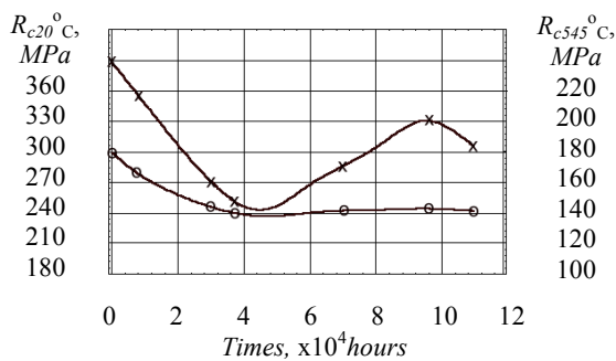
Fig. 6. Dependence of yield strength on time of operation: o – the research was done at the 20 °C temperature, × – the researches was done at the 545 °C temperature
