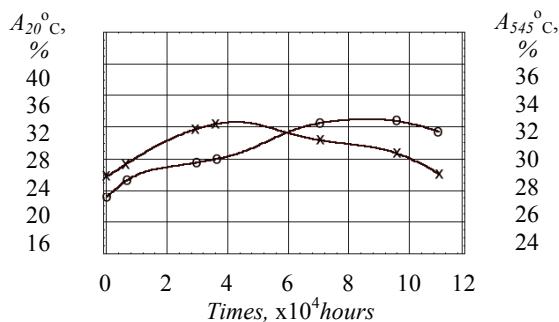
Fig. 7. Dependence of elongation on time of operation: o – the research was done at the 20 °C temperature, × – the researches was done at the 545 °C temperature
