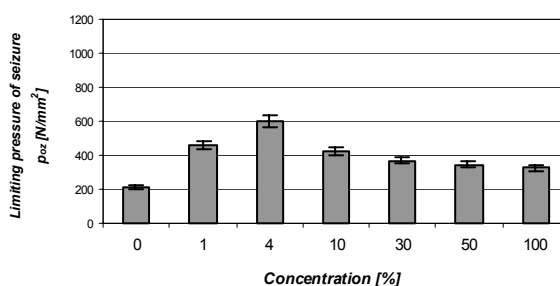
Fig. 9. Limiting pressure of seizure p_{oz} versus concentration of water solutions of ethoxylated sorbitan monooleate
