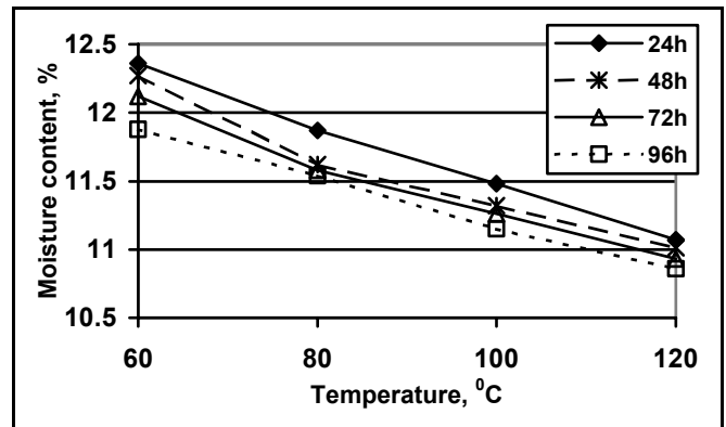
Fig. 2. Relationships of mean actual moisture content with respect to thermotreatment temperature and time (outside, summer)
