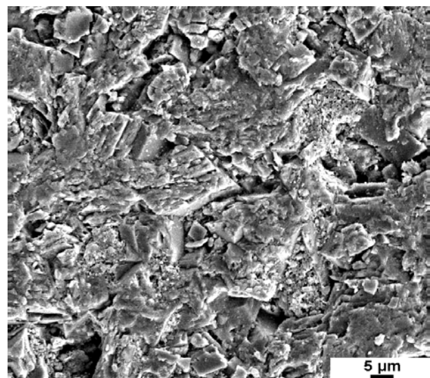
Fig. 8. Chemically etched surface of Orgita dolostone shows a dense structure. SEM microphoto
