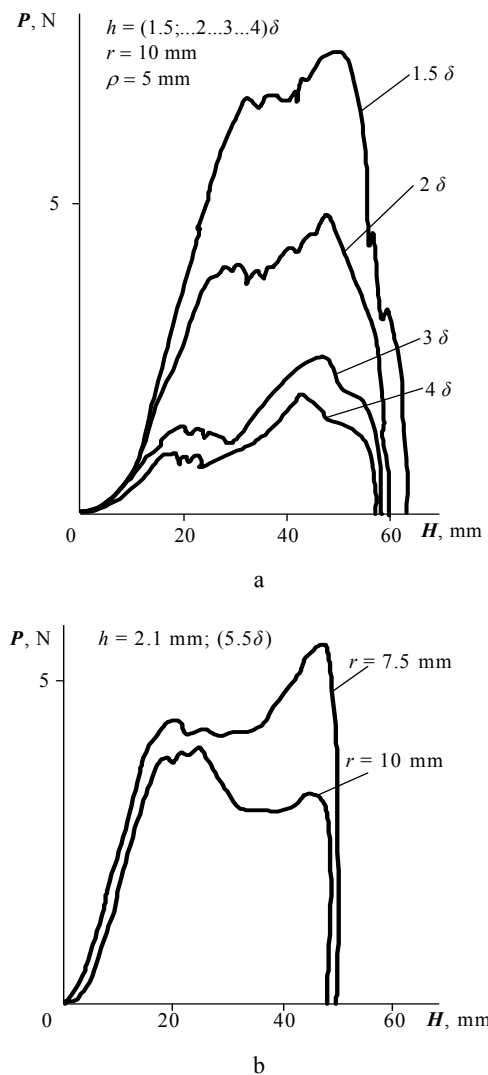
Fig. 3. Typical pulling curves H-P : a – when the distance between the limiting plates varies in the range from 1.5 \delta up to 4 \delta (fabric R); b – for different radiuses r of the hole (fabric G-2)
