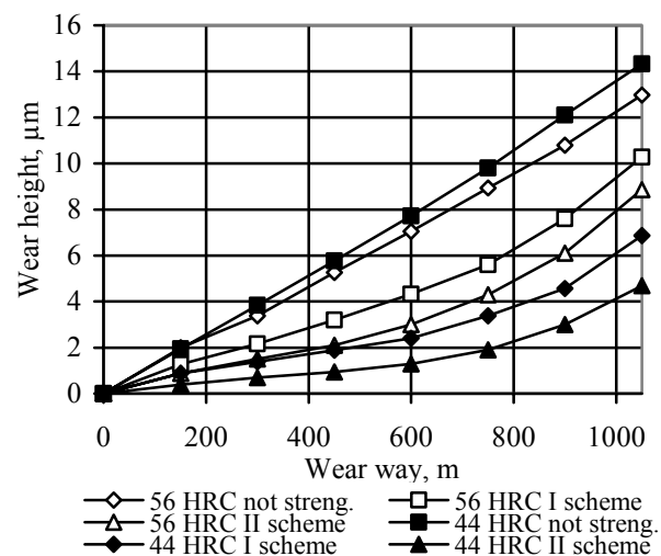
Fig. 4. Wear resistance of the test pieces prepared from X12Φ1 steel
