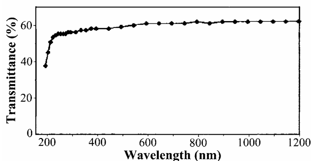
Fig. 10. The transmittance spectrum of Y_3Sc_2Al_3O_{12} garnet sample
