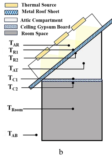
Fig. 4. Testing configuration: a – schematic representation of the testing model setup; b – configuration of fixed thermocouple positions in the model without the PCM layer
