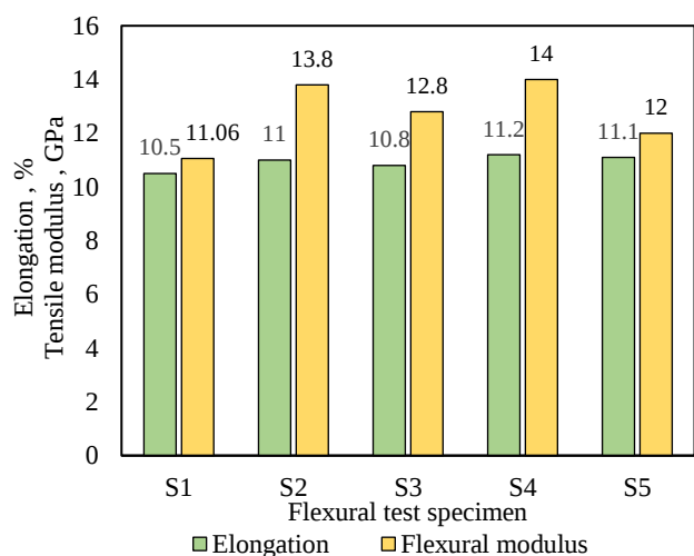
Fig. 5. Elongation and flexural modulus of composite
