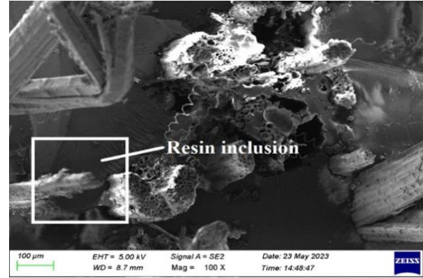
Fig. 10. Tensile fracture image
