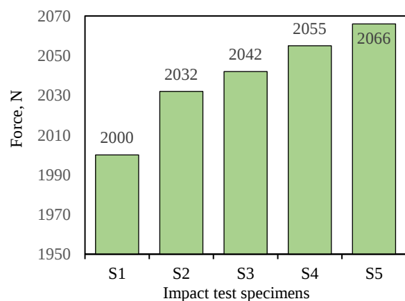
Fig. 7. Impact force hybrid composite
