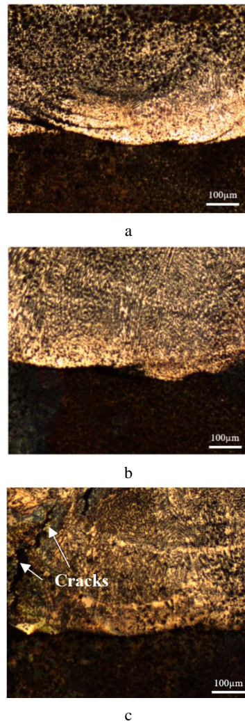
Fig. 2. Metallographic photos of DLD 50Cr6Ni2Y coatings with different TiC contents: a–1#; b–2#; c–3#
