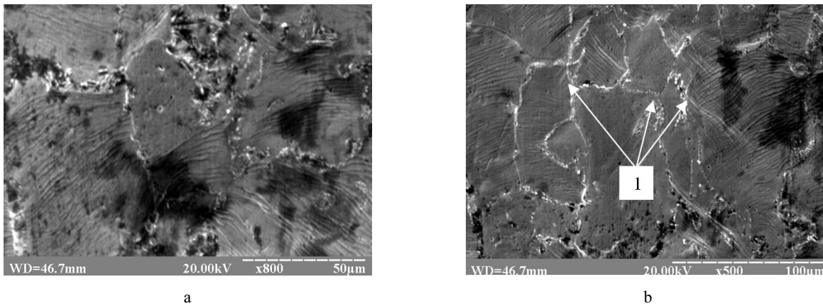
Fig. 6. Structure of boundaries of steel 25Kh1M1F ( N = 200 cycles) after cyclic loading; 1 – pores; plastic shears and turns of grain conglomerates are pointed with arrows
