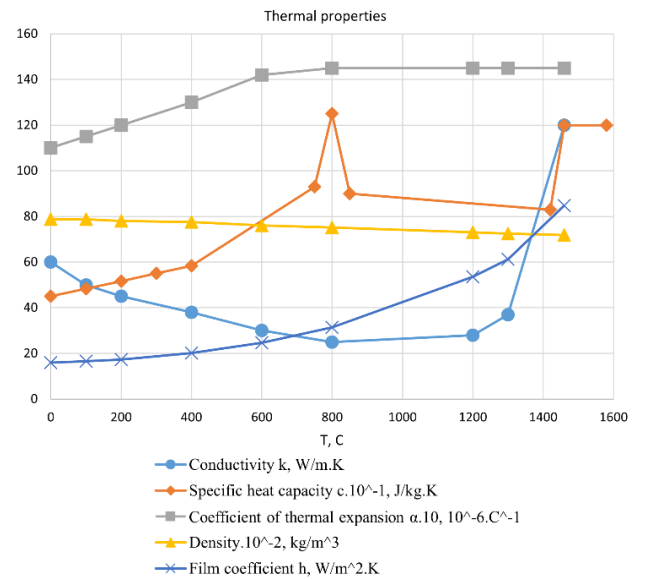
Fig. 8. Thermal properties of the SS400 steel plate [16, 17]
