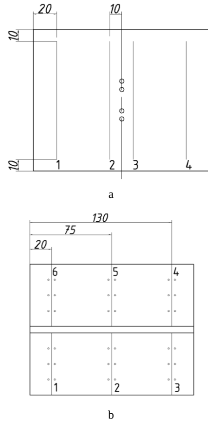
Fig. 7. a – lines for straightness measurement on the bottom surface of the flange; b – points for local plane approximation on the flange surface and the same for the web surface, in total measuring 3 angles on each side
