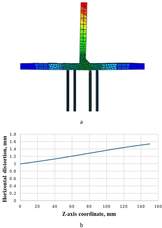
Fig. 13. a – the deformation of 1-side welding; b – horizontal distortion distribution along the welding line
