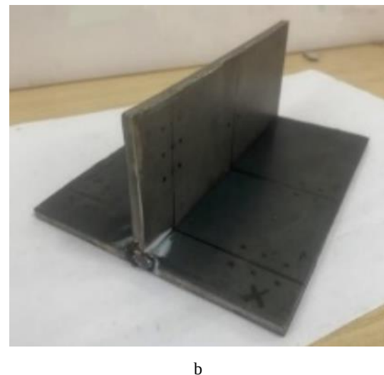
Fig. 1. The welding experimental model: a – specimen's dimensions and coordinates; b – real experiment specimen
