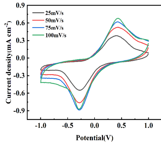
Fig. 5. CV at different scan rates from 25 \text{ mVs}^{-1} to 100 \text{ mVs}^{-1}
