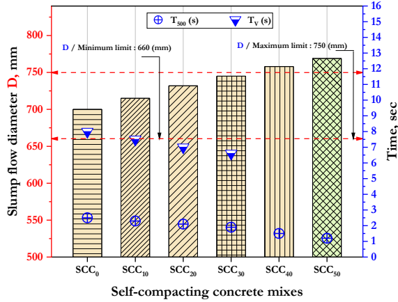
Fig. 9. Slump flow diameter, T500, and Tv of SCC mixes
