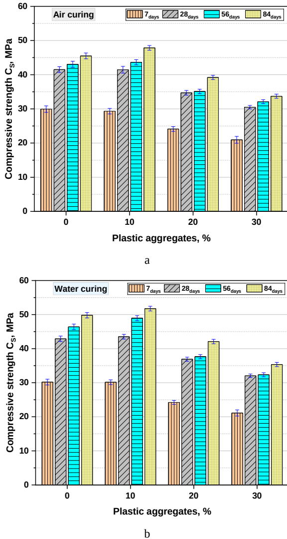
Fig. 15. Effects of plastic aggregates on the compressive strength of all SCC: a – under air; b – under water curing conditions
