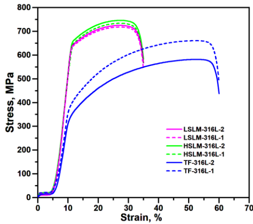
Fig. 5. Tensile stress-strain curves of the SLM-316L and TF-316L samples
