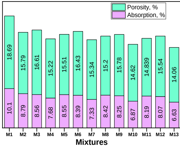
Fig. 5. Absorption and porosity of mixtures (after 28 days)
