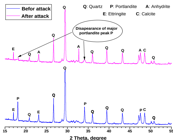
Fig. 8. The XRD spectra before and after the attack of \text{H}_2\text{SO}_4
