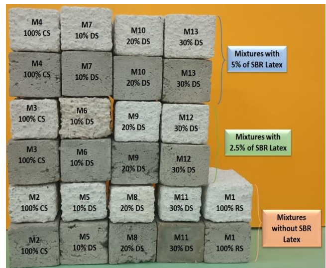
Fig. 7. Samples of degradation of different mixtures after 60 days of attack by 5 % H_2SO_4
