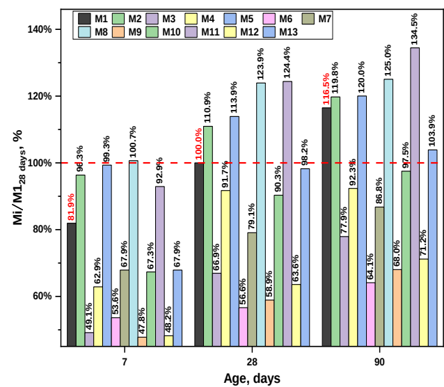
Fig. 4. Compressive strength ratio of the mortars as a function of M1 28 days
