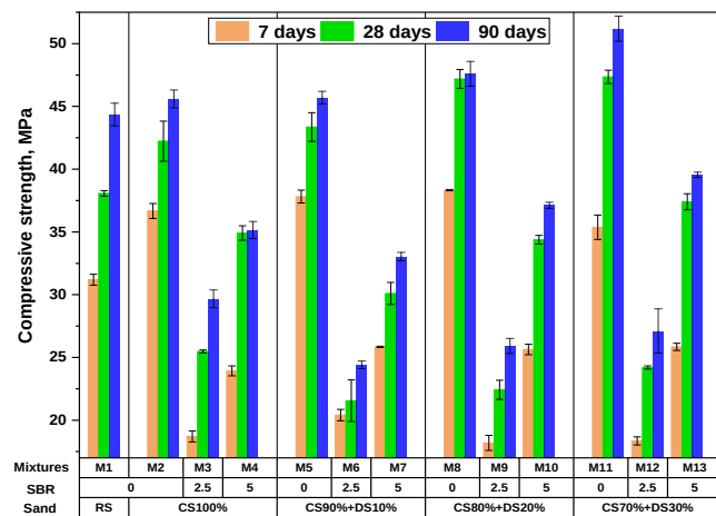
Fig. 3. Compressive strength of the mortars versus SBR latex and sands
