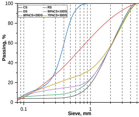
Fig. 1. Sieve analysis of sands
