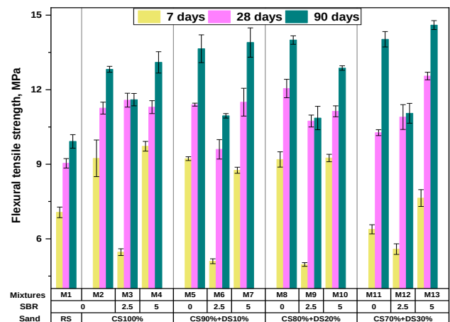
Fig. 2. Tensile strength of the mortars versus SBR latex and sand
