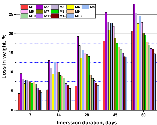
Fig. 6. Mass loss of mixtures as a function of immersion time for 5% H_2SO_4
