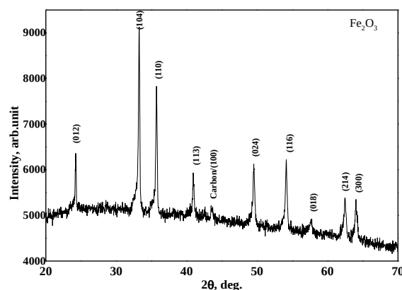
Fig. 1. XRD pattern of the AC doped \text{Fe}_2\text{O}_3 nanoparticles
