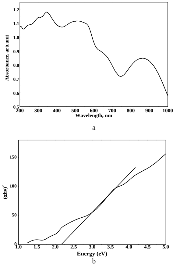
Fig. 3. UV-visible spectroscopy studies of the AC doped \text{Fe}_2\text{O}_3 sample: a – absorption spectra; b – Tauc plot
