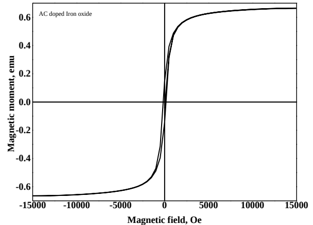
Fig. 4. Magnetisation (M-H) curve of AC doped \text{Fe}_2\text{O}_3 nanoparticles
