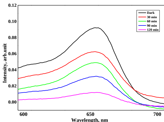
Fig. 5. Photocatalytic degradation of MB dye using AC-Fe 2 O 3 catalyst
