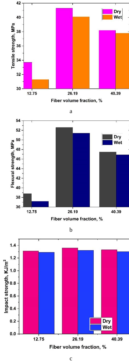
Fig. 7. Mechanical properties: a–tensile; b–flexural; c–impact of composite exposed to the distilled water environment
