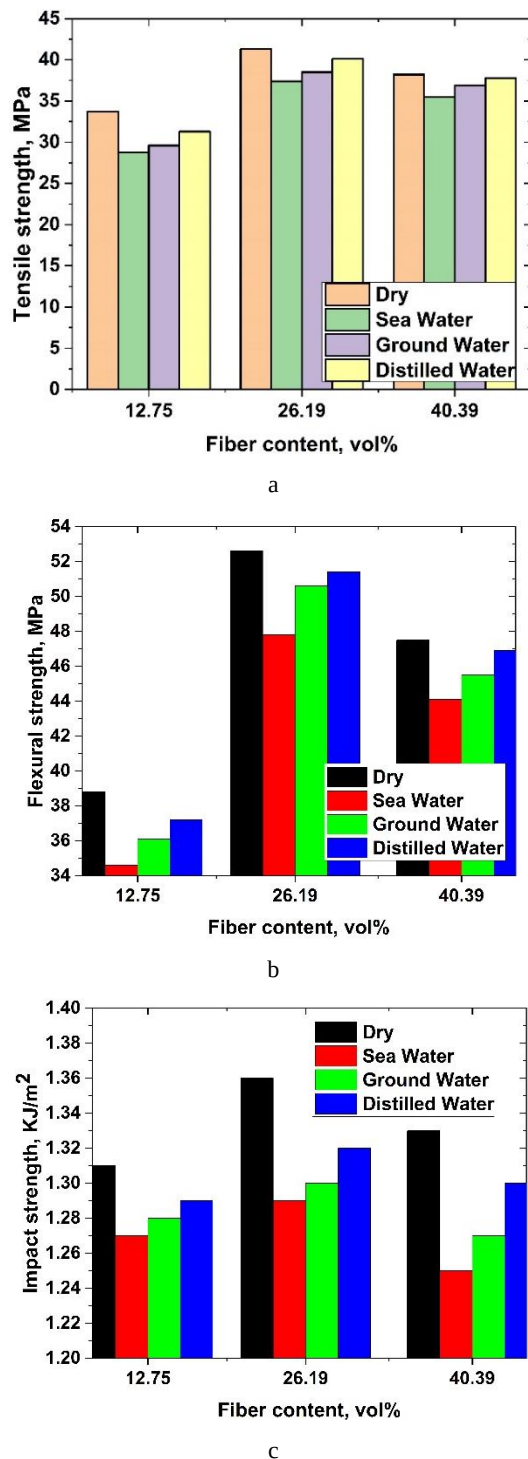
Fig. 9. Comparison of mechanical properties: a–tensile; b–flexural; c–impact of composite exposed to the sea, ground, and distilled water environments
