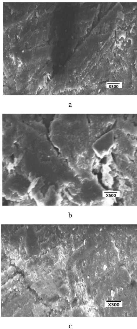
Fig. 6. SEM images of the tensile fracture surface of composite exposed to the groundwater environment
