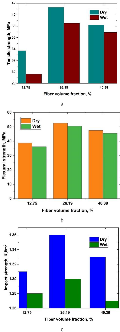
Fig. 5. Mechanical properties: a – tensile; b – flexural; c – impact of composite exposed to the ground water environment
