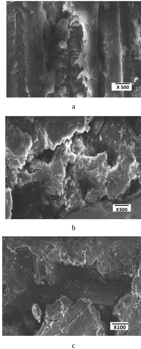
Fig. 4. SEM images of the tensile fracture surface of composite exposed to the seawater environment
