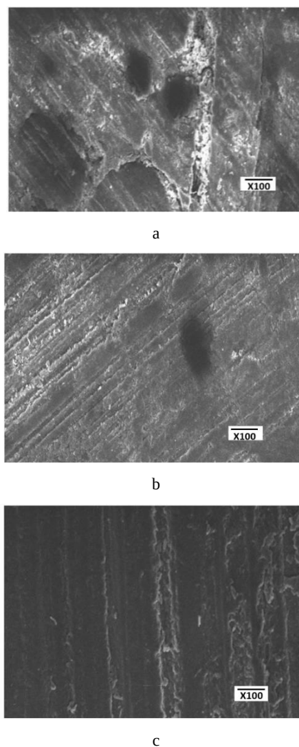
Fig. 8. SEM images of the tensile fracture surface of composite exposed to the distilled water
