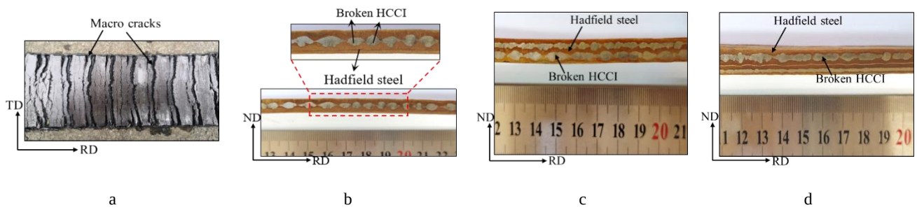
Fig. 3. Macromorphology of the sheet after hot rolling: a – single HCCI; b – three layer slab; c – five layer slab; d – seven layer slab
