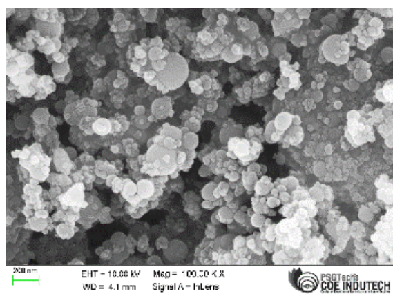
Fig. 5. Scanning electron microscopic image of SiO 2 : a—at 100 rpm 2 h; b—at 100 rpm 4 h; c—at 200 rpm 2 h; d—at 200 rpm 4 h; e—at 300 rpm 2 h; f—at 300 rpm 4 h
