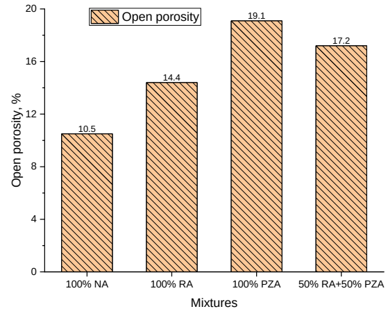
Fig. 4. Effect of different types of aggregates on the open porosity
