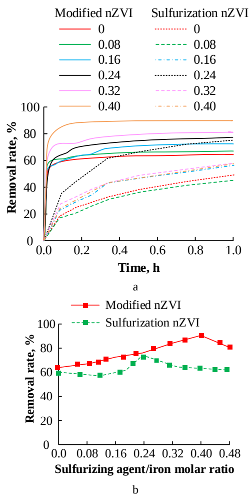
Fig. 8. Effect of sulfurizing agent-to-iron molar ratio on the properties of modified nZVI nanomaterials: a – variation in removal rate over time; b – removal rate as a function of sulfurizing agent-to-iron molar ratio
