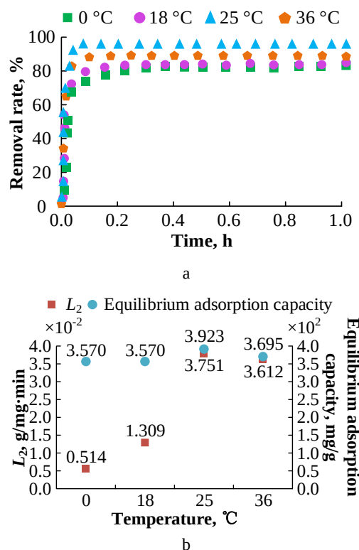
Fig. 10. Effect of temperature on the removal efficiency and reaction kinetics of modified nZVI nanomaterials: a – impact on removal efficiency; b – impact on reaction kinetics
