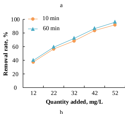
Fig. 11. Effect of dosage on the removal performance of modified nZVI nanomaterials: a – impact on hexavalent chromium concentration; b – impact on removal rate
