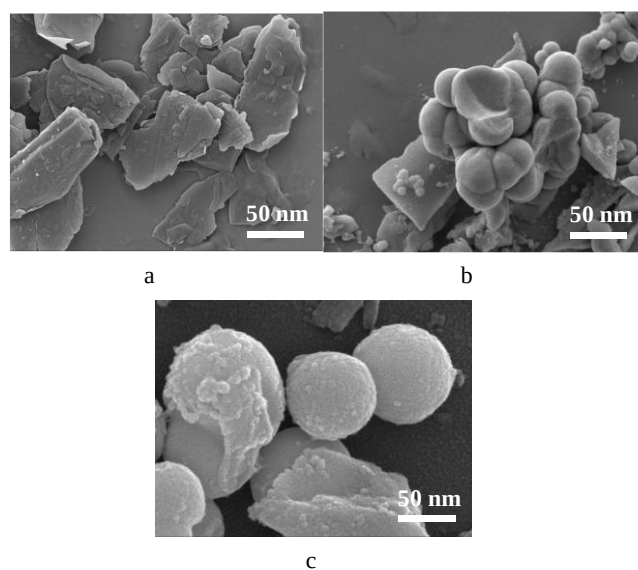
Fig. 2. SEM images of modified nZVI nanomaterials synthesized using three different methods: a – pre-sulfurization method; b – surface deposition method; c – surface corrosion method
