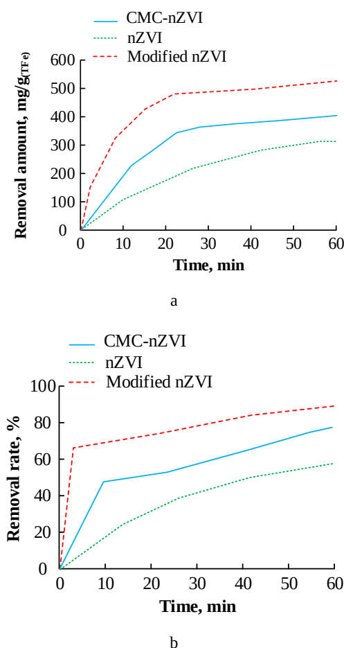
Fig. 15. Removal performance of modified nZVI nanomaterials on Cr(VI) in simulated wastewater: a—variation in Cr(VI) removal over time; b—variation in Cr(VI) removal rate over time
