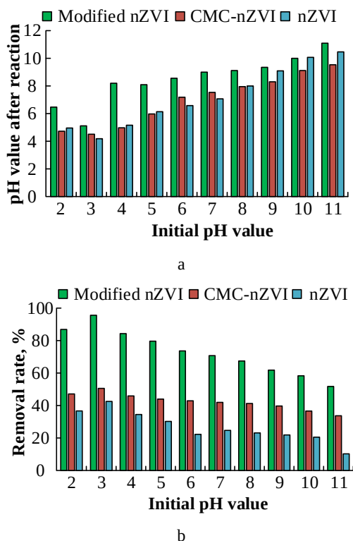
Fig. 9. Comparison of the effect of initial pH on the removal efficiency of different materials: a – effect of initial pH on the pH value after the reaction; b – effect of initial pH on the removal efficiency
