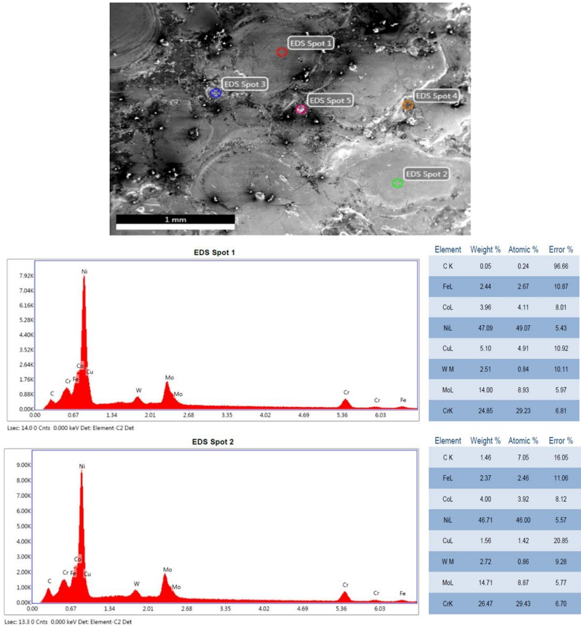
Fig. 1. SEM of Hastelloy machined surface processed in Cu-incorporated dielectric medium
