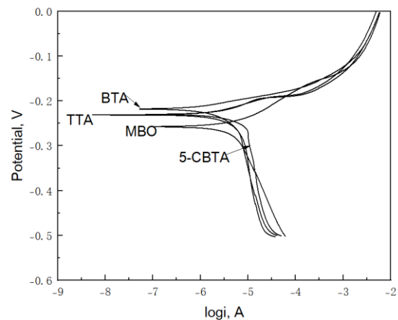
Fig. 3. Tafel diagrams of copper sheets exposed to 3.5 % NaCl solution with various corrosion inhibitors
