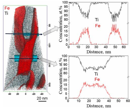
Fig. 11. 3-D APT reconstruction showing Fe (red) and Ti (black) atoms, the red surface represents an isoconcentration surface of 4 at% Fe (threshold value); 1-D concentration profiles through the \beta lamella of Ti-3% Fe 950 °C + 550 °C-WQ [91]
