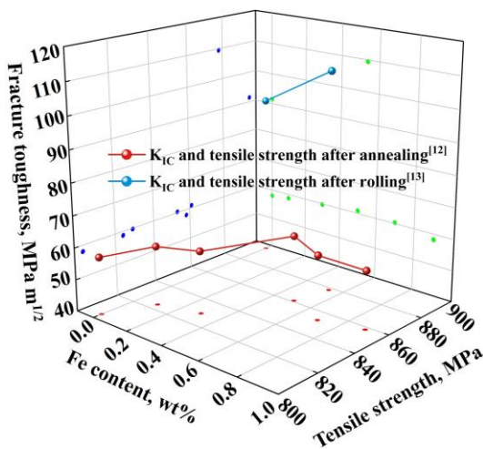
Fig. 9. Relationship between tensile strength and fracture toughness of Fe microalloying TC4 alloy. Data were collected from Ref. [12, 13]
