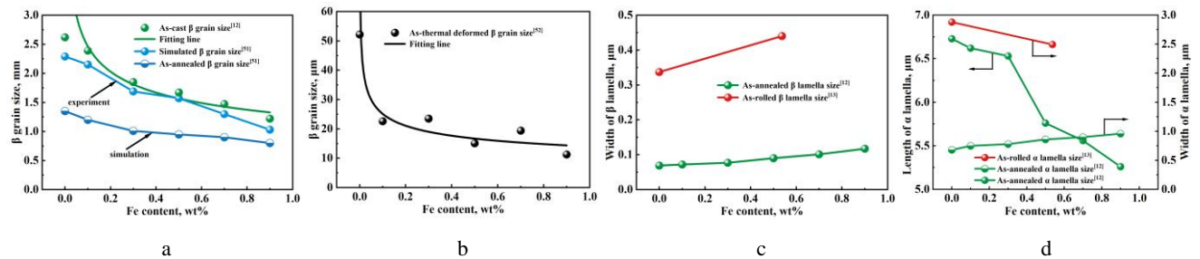
Fig. 5. Dependency of grain sizes of TC4 alloy on Fe content: a- \beta grain size; b- \beta grain size after deformation; c- width of \beta lamella; d-length and width of \alpha lamella. Data were collected from Ref. [12, 13, 51, 52]
