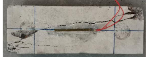
Fig. 4. Uniaxial compression failure mode
