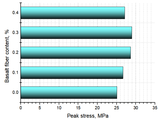
Fig. 6. Peak stress
