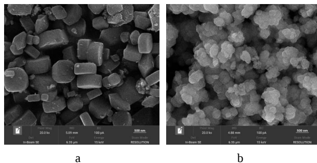
Fig. 5. The SEM image: a – \text{NH}_2\text{-MIL-125(Ti)} ; b – \text{NH}_2\text{-UIO-66(Zr)}
