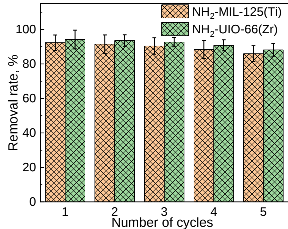
Fig. 14. Adsorption and regeneration properties of NH 2 -MIL-125(Ti) and NH 2 -UIO-66(Zr)
