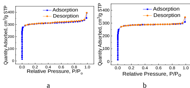
Fig. 8. The BET spectra: a – \text{NH}_2\text{-MIL-125(Ti)} ; b – \text{NH}_2\text{-UIO-66(Zr)}
