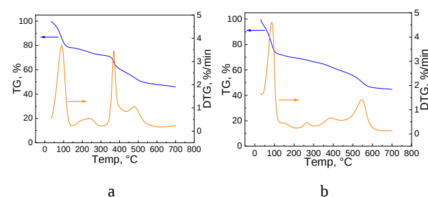
Fig. 9. The TGA spectra: a – \text{NH}_2\text{-MIL-125(Ti)} ; b – \text{NH}_2\text{-UIO-66(Zr)}
