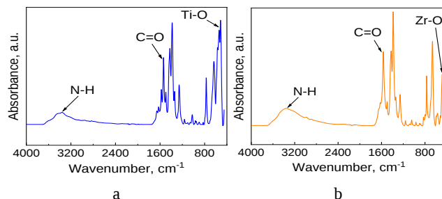
Fig. 6. The FTIR spectra: a – \text{NH}_2\text{-MIL-125(Ti)} ; b – \text{NH}_2\text{-UIO-66(Zr)}
