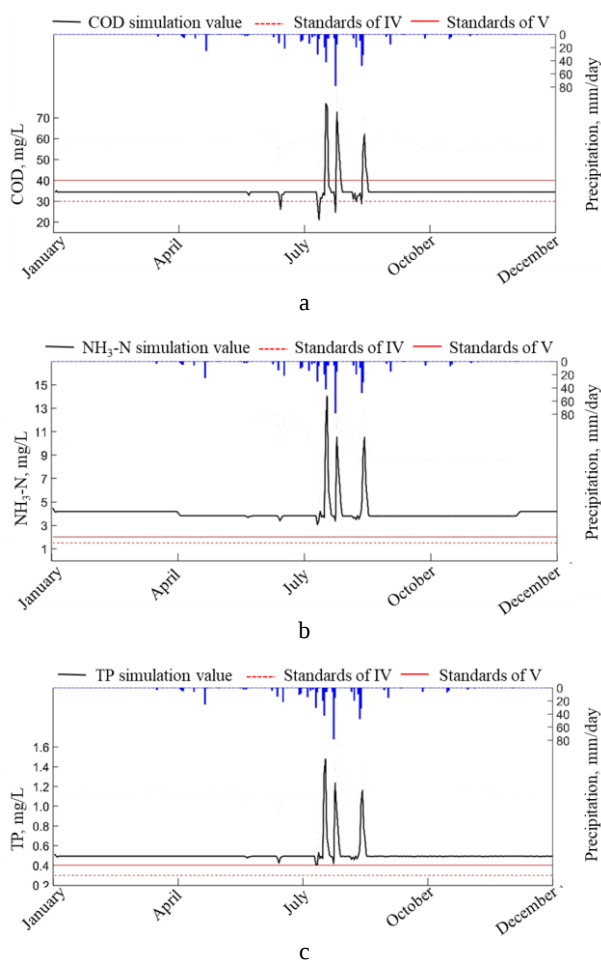
Fig. 3. Annual simulation diagram of water quality concentration dynamics at the section of Shaobingzhuang sluice in the water supply project: a – COD; b – \text{NH}_3\text{-N} ; c – TP
