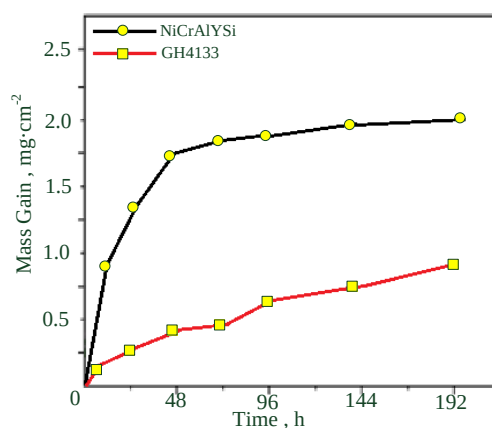
Fig. 6. Coating kinetics curve
