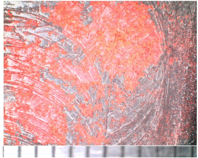
Fig. 13. Hatched corroded areas of the third corroded surface (distance between vertical lines is ~1 mm) – changed hatching parameters in the Python code
